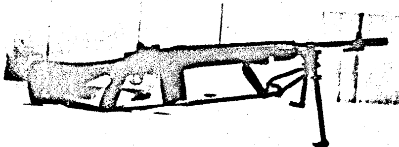
M14E2 Automatic Rifle
