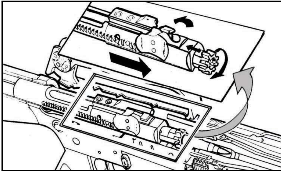
Figure 4-4. Locking.
