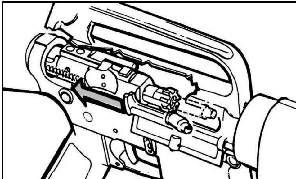
Figure 4-8. Ejecting.
