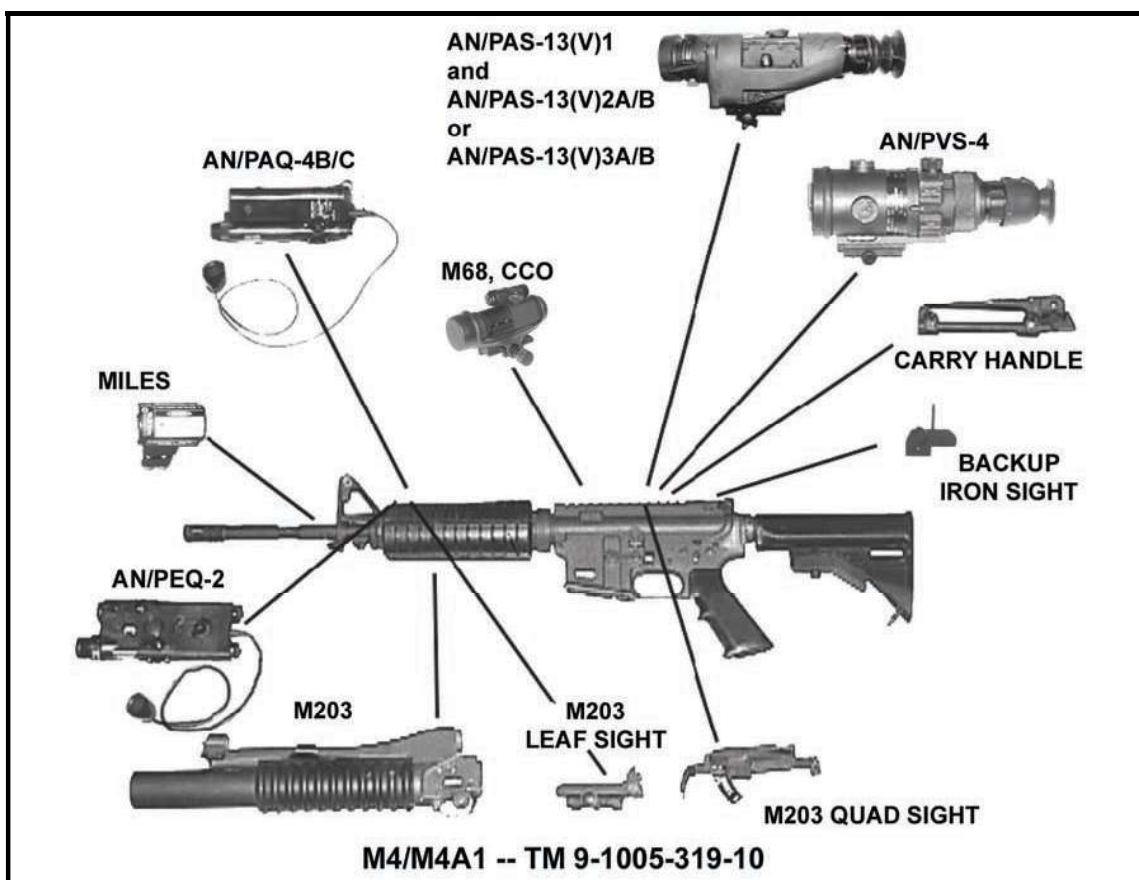
Figure 2-1. M4/M4A1 carbine with accessories.
