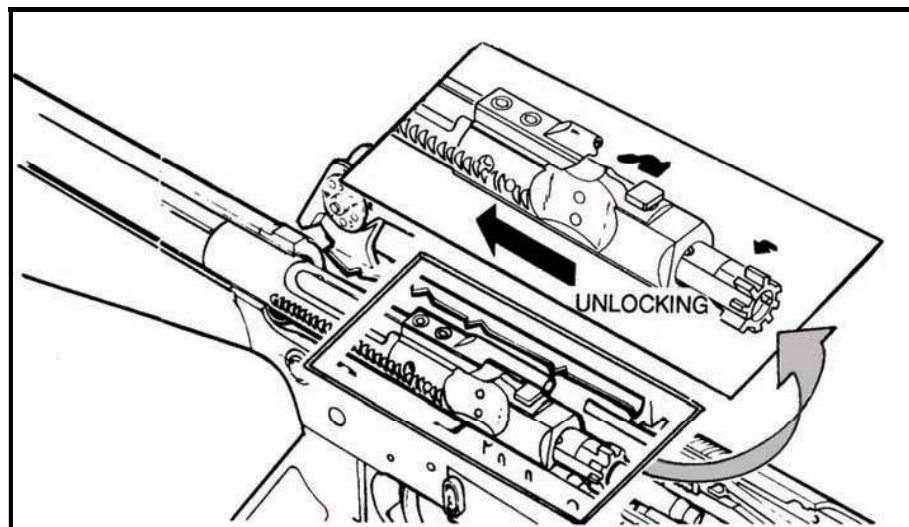
Figure 4-6. Unlocking.
