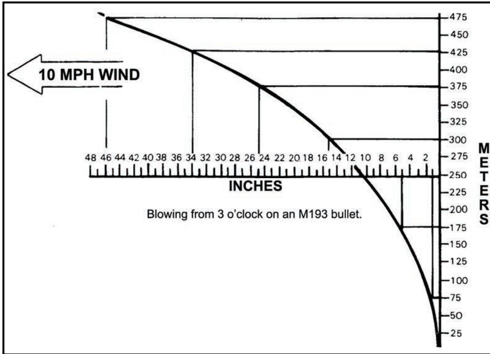
Figure 5-29. Calculate the adjusted point of aim based on wind speed.
